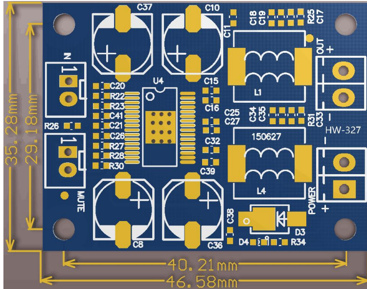
PCB front side:
